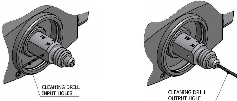
Cleaning "Round" Chamber Product Input Holes
